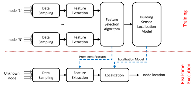
Fig. 1. Overall data processing flow: training phase and real-time execution of the sensor localization algorithm
