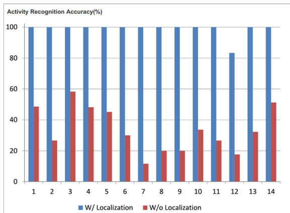
Fig. 4. Accuracy of activity recognition for individual movements with and without sensor localization
