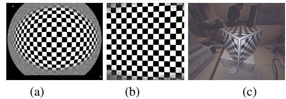
Fig. 4. Calibration of endoscopic camera: (a) map from monitor to endoscopic camera image, (b) undistorted map (only 2D projective transformation map remains), and (c) calibration object (undistorted).
