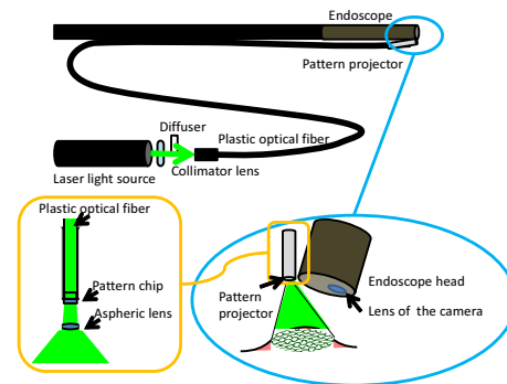
Fig. 1. 3D endoscope system
