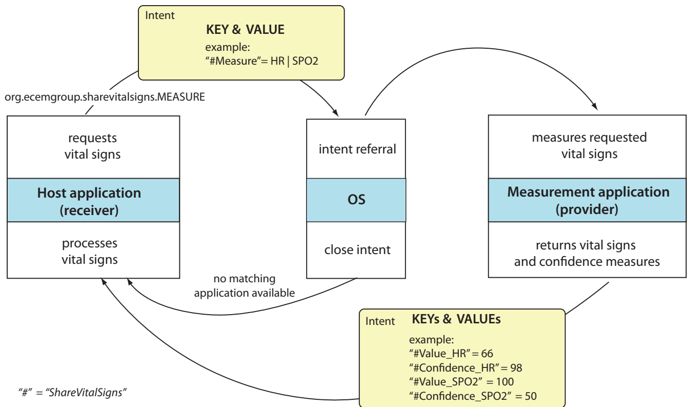
Fig. 2. Steps to request a vital sign using the ShareVitalSigns library. The host application is opening an intent with a measure field containing the requested vital sign. The Android OS then provides a list of applications that provide the requested vital sign. If an application is chosen, the intent is referred to the chosen measurement application. After the measurement, the intent is returned with new key and value pairs for the measured vital signs.
