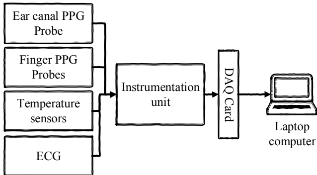
Figure 1: Block diagram of the measurement system.
