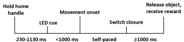
Fig. 1. Each successful task conforms to the shown timeline. From movement onset, the monkey has 10 s to reach to the correct object and close the switch before the trial is aborted and labeled a failure.
