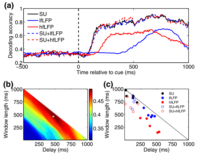
Fig. 3. (a) Decoding accuracy over time is plotted between 3 distinct reach and grasp movements for each of the decoders constructed. Each line represents an average over the 5 cross-validation folds. (b) An example of a parameter map to identify the optimal delay ( t_0 ) and time window ( w ) parameters for the lfLFP decoder, where color represents the average decoding accuracy over the 1000 ms window following cue presentation. The white asterisk represents the ( t_0 , w ) pair that maximizes decoding accuracy in the validation set and was thus chosen for this particular lfLFP decoder. (c) All ( t_0 , w ) parameter pairs chosen for each decoder. Five points per decoder correspond to each of the decoders constructed using 5-fold cross validation.
