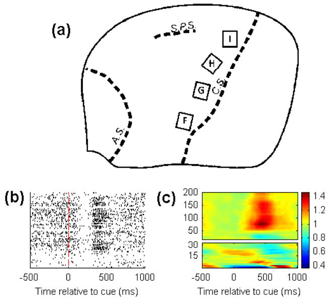
Fig. 2. (a) Arrays F, G, H, and I were implanted anterior to the central sulcus in the putative arm and hand area of M1. (b) A raster plot of a characteristic spike for all sphere trials. (c) The average relative power spectrogram for all successful sphere trials taken from the same electrode. The relative power spectrogram was calculated by dividing the power at each frequency and timepoint by the baseline power at each frequency, where baseline power was defined as the average power from -500 ms to 0 ms for all trials of a particular type.
