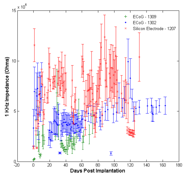
Figure 1. Chronic Impedance Magnitude. The 1 kHz impedance of contact
