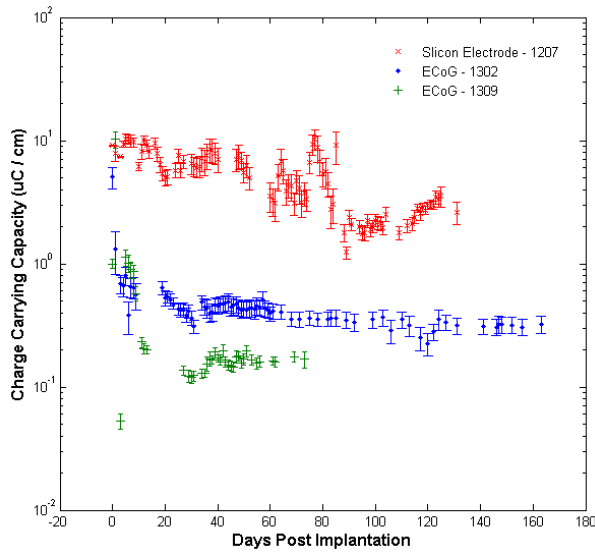
Figure 2. Chronic charge carrying capacity of \mu ECoG arrays (Blue, Green) and a penetrating electrode (Red) over time post implantation. Error bars show standard error.
