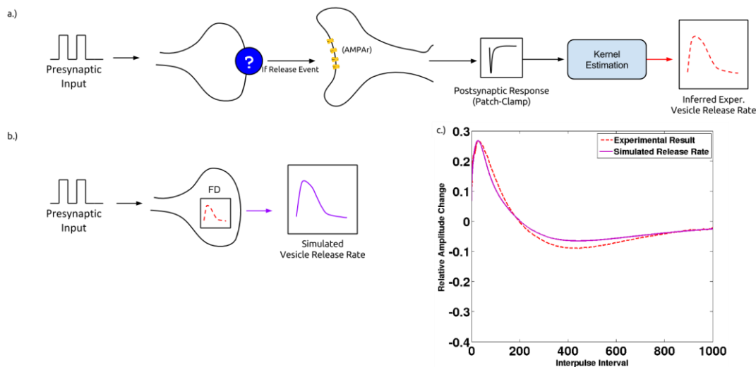
Figure 1. Calibration of the Presynaptic Release Model based on Experimental Data. (a) the vesicle release rate was inferred from experimental data by analyzing kernel responses from patch clamp experiments, according to [1]. Release events are captured through postsynaptic responses, which are then analyzed through Volterra kernel estimation techniques. (b) The Facilitation/Depression (FD) model from [2] was calibrated with the inferred probabilistic release rate derived from the experimental data. (c) a comparison between the experimentally derived release rate (dashed) and the (calibrated) simulated release rate (solid). The graph shows the change in amplitude of a 2 nd event relative to the 1 st event response based on the time interval elapsed between the two events.
