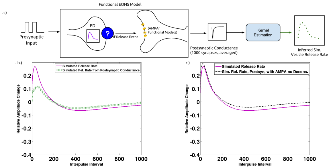
Figure 2. Simulations using the EONS functional model. (a) Representation of the EONS functional model and simulation techniques for estimating vesicle release rate. Postsynaptic responses were analyzed similar to the experimental setup as explained in Fig 1. The Functional EONS model utilizes the FD model calibrated from Fig. 1 and AMPA receptor models based on AMPA receptor kinetics. (b) comparison between the simulated release rate from the FD model (solid) and the inferred release rate from the kernel estimation of the postsynaptic response (dotted). (c) uses the same setup as (a) except that the kinetics of the AMPA receptors were modified such that AMPA receptor desensitization was inhibited (results shown in the dash-dotted line).
