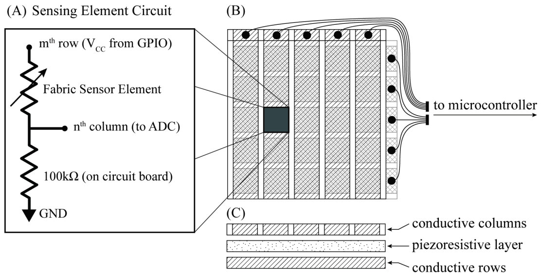
Figure 2. (A) Each element in a fabric sensor array is connected in series with a 100\text{k}\Omega resistor to create a variable resistor divider. The microcontroller scans through each element in the m \times n array to sample a pressure reading. (B) Top view of fabric sensor array. (C) Side view of fabric sensor array.
