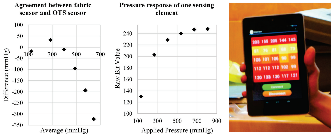
Figure 3. Left: A Bland-Altman plot showing agreement of fabric sensor to a commercial sensor. Middle: Extended pressure response of a single sensing element showing limitations in dynamic range. Raw bit values from measurement range from 0-255. Right: Measurement output when the fabric sensor is placed on a cushioned chair and a human sits on the sensor. Raw bit values on each square represent pressure values from the sensor.
