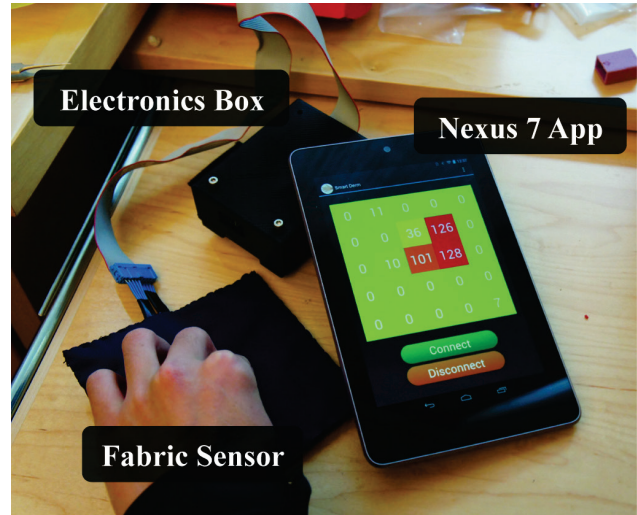
Figure 1. Pressure on the fabric sensor is acquired and digitized by the microcontroller in the electronics box, then transmitted over Bluetooth v2.1 to an Android application running on a Nexus 7 device. The next iteration of this device will involve miniaturization of the electronics box and use of Bluetooth Low Energy technology.
