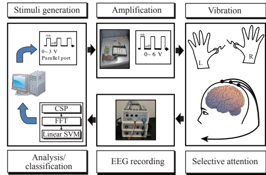
Fig. 1. Overview of the SSSEP-based BCI system
