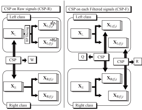
Fig. 3. Two methods for applying the CSP for the SSSEP classification
