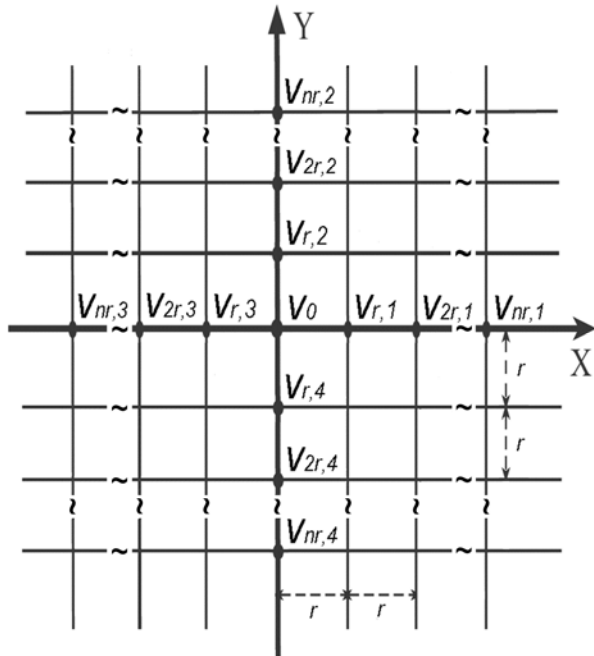
Figure 2. Regular plane square grid with interpoint distance equal to r .
