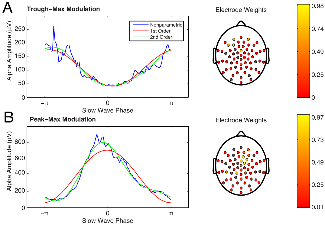
Fig. 1 For trough-max modulation (A), and peak-max modulation (B), estimates of the empirical phase/amplitude relationship (blue) are shown along with first and second order model fits. The optimal weights for each electrode are shown to the right as estimated by the cost minimization procedure using the sinusoidal model of order 1 for trough-max and order 2 for peak max, chosen based on the corresponding F-statistics.
