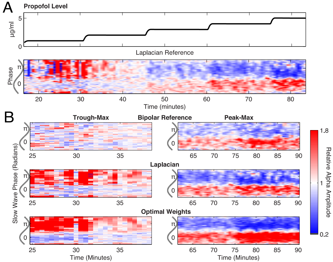
Fig. 2 (A) The targeted effect-site propofol concentration is shown, along with the time-varying phase-amplitude histogram computed based on Laplacian-referenced data for a period spanning the trough-max and peak-max phase regimes of modulation. (B) Phase-amplitude histograms computed separately for a bipolar referencing, Laplacian referencing, and using the optimized combination of electrodes for both trough-max and peak-max data segments.
