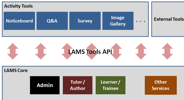
Figure 2. Architecture of the training application as [14].
