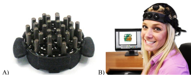
Figure 1. A) Hybrid sensors for through-hair measurement of EEG B) QUASAR headset on subject.
