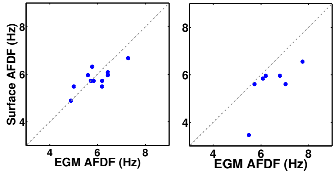
Fig. 2. EGM/surface AFDF correlation for terminating patients (left) and non-terminating patients (right). The dash-dotted line represents x = y .
