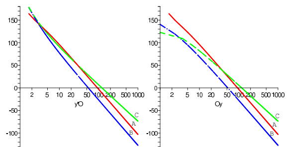
Figure 11: External relative sensitivity along the two halves of the Oy axis for (A) a tripolar cuff electrode, (B) a planar hexagonal patch and (C) a bent hexagonal patch. The vertical axis is in \text{dB} and the unit for the horizontal axis is the radius R of the electrode.
