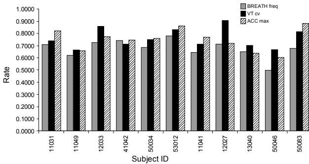
Fig. 3. Validation rate for the best predictors from the combined SW models.
