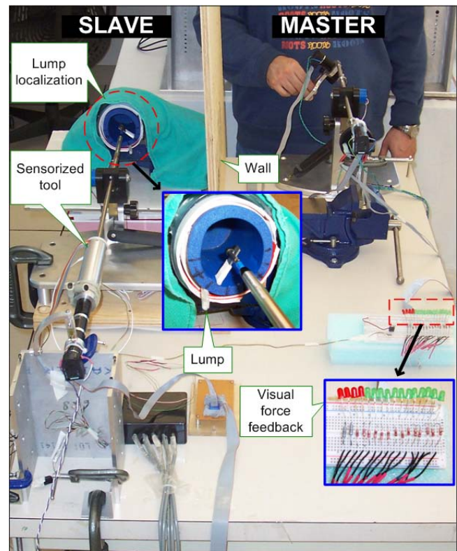
Fig. 1. Setup for telemanipulated lump localization.
