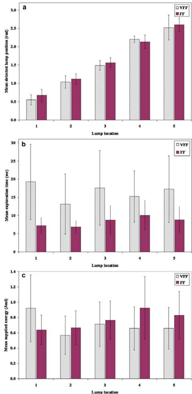
Fig. 2. (a) Mean detected lump position (rad); (b) mean exploration time (sec); (c) mean energy supplied to the tissue (Jou). Error bars show standard deviations.
